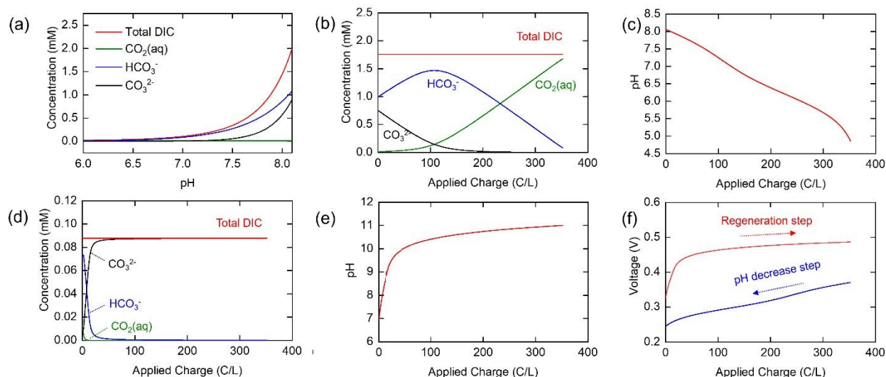
Fig. 2. (a) Equilibrium concentration of inorganic carbon species ( \text{CO}_2 , \text{HCO}_3^- , \text{CO}_3^{2-} ) and total DIC at pH 6-8.1 in simulated seawater and estimated equilibrium concentration of each ionic species in simulated oceanwater in pH decrease step ((b) \text{HCO}_3^- , \text{CO}_3^{2-} , and total DIC, and (c) pH of oceanwater) and in the regeneration step ((d) \text{CO}_2 , \text{HCO}_3^- , \text{CO}_3^{2-} , and total DIC, and (e) pH during the regeneration step. (e) Equilibrium voltage vs. charge curve of chloride-mediated electrochemical pH swing system for \text{CO}_2 removal based on the thermodynamic modeling.
