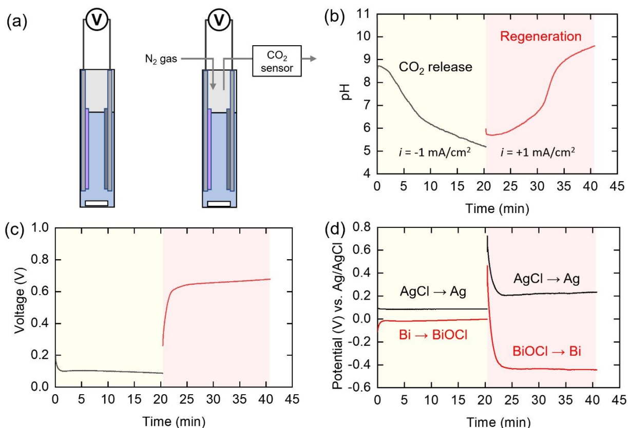
Fig. 4. Electrochemical results and pH profile monitored during CO_2 release step (yellow) and re-alkalization step (pink) in the pH swing operation using a static cell. (a) Electrochemical cell exposed to ambient air, and closed with nitrogen sweep stream, (b) pH change of the electrolyte, (c) voltage profile, and (d) electrochemical potential of individual electrodes.
