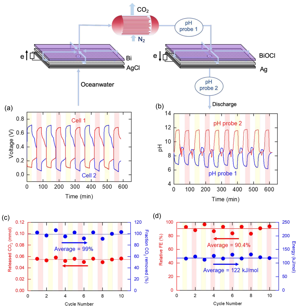
Fig. 5. Profiles monitored during the continuous electrochemical pH swing process operation for 10 cycles. (a) Voltage and (b) pH of the effluents from two cells. (c) Molar amount of released \text{CO}_2 (red, left) and fraction of \text{CO}_2 removed (blue, right). (d) Relative Faradaic efficiency (red, left) and energy consumption (blue, right) during the operation of continuous process for 10 cycles.
