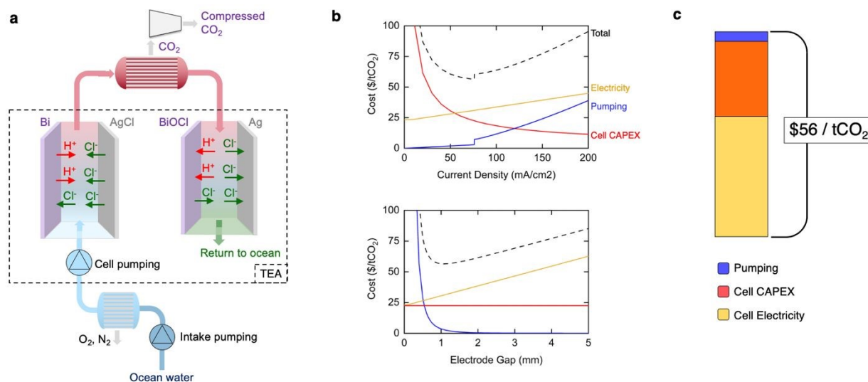
Fig. 8. (a) Complete DOC system including intake systems, gas separations, and compression. The scope of this TEA is shown by the dashed box, including cell stack costs, electricity, and pumping. (b) System cost optimization of cell current density and inter-electrode gap. When current density is varied, electrode gap is fixed at 1.1 mm. When electrode gap is varied, current density is fixed at 76 mA/cm 2 . (c) System cost components at a current density of 76 mA/cm 2 and an inter-electrode gap of 1.1 mm where total costs are minimized at $56/tCO 2 .
