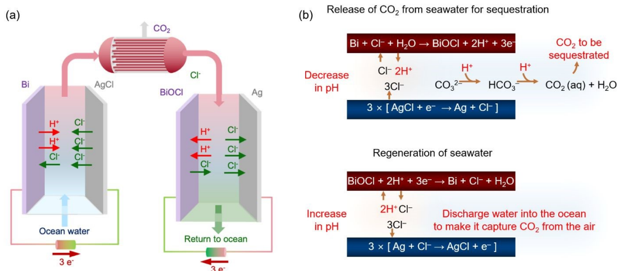
Fig. 1. (a) General principle of the chloride-mediated electrochemical pH swing system for CO 2 removal from ocean water. (b) Electrochemical reactions at bismuth (red) electrode and silver (blue) electrode in each step, and subsequent CO 2 release in the acidified oceanwater.
