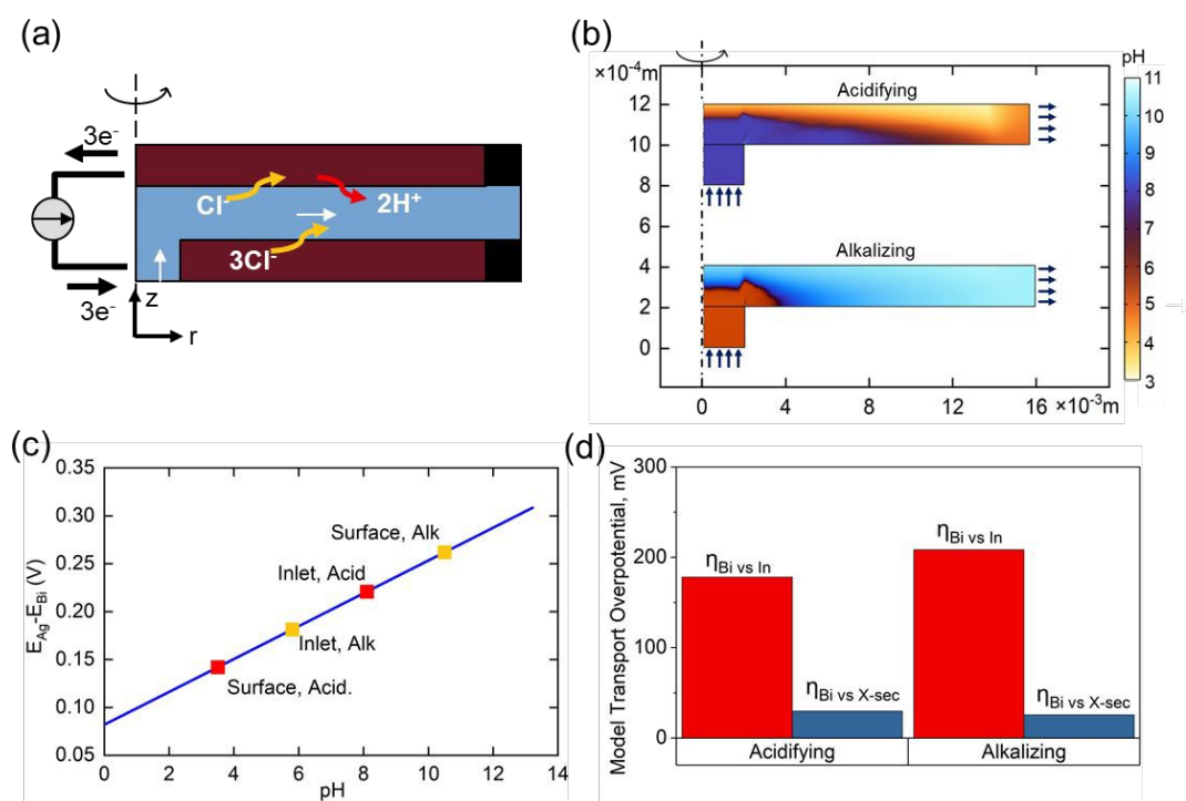
Fig. 6. COMSOL transport model and results (a) simulated flow cell geometry during acidification (b) pH profile of the simulated cell during steady state operation (c) dependence of open circuit potential on pH (d) total measured Bi/BiOCl overpotential ( \eta_{\text{Tot}} ) in the flow cell compared to model predictions of polarization overpotential relative to inlet ( \eta_{\text{Inlet}} ) and polarization relative to average cross section pH ( \eta_{\text{X-sec}} )
